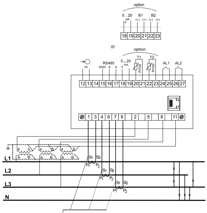
Indirect measurement in 4-wire network - connection of input signals
