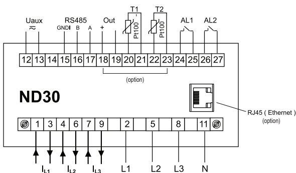
Description of meter connections strips
