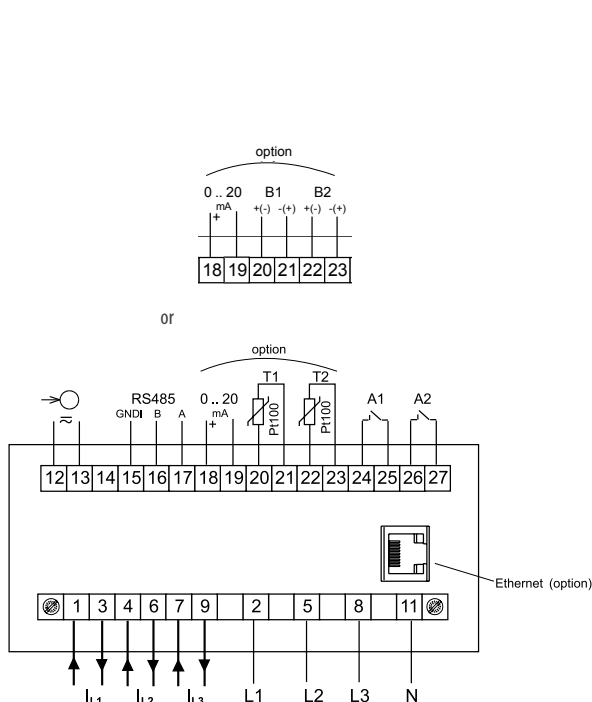
Description of meter connections strips
